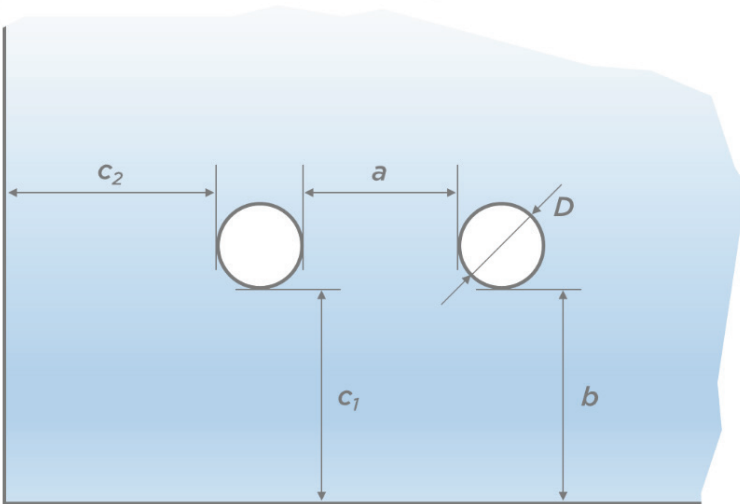
Picture 17: Position of the holes
