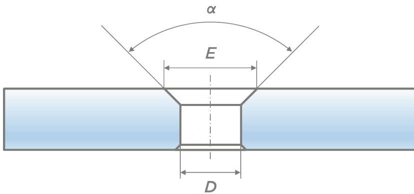
Picture 14: Countersunk hole
