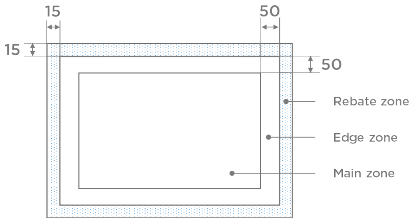
Picture 28: Zones for the assessment of visual quality according to ÖNORM EN 1279-1 [dimensions in mm]
