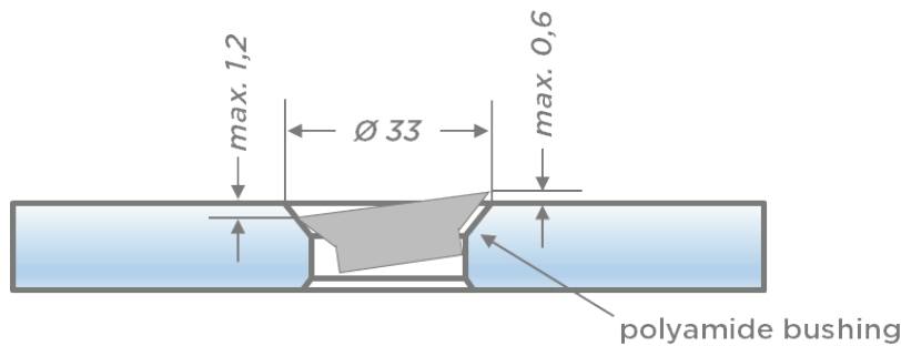
Picture 30: Schematic representation of possible mounting positions of e.g. LITE-WALL fittings, 90° countersunk [Dimensions in mm]
