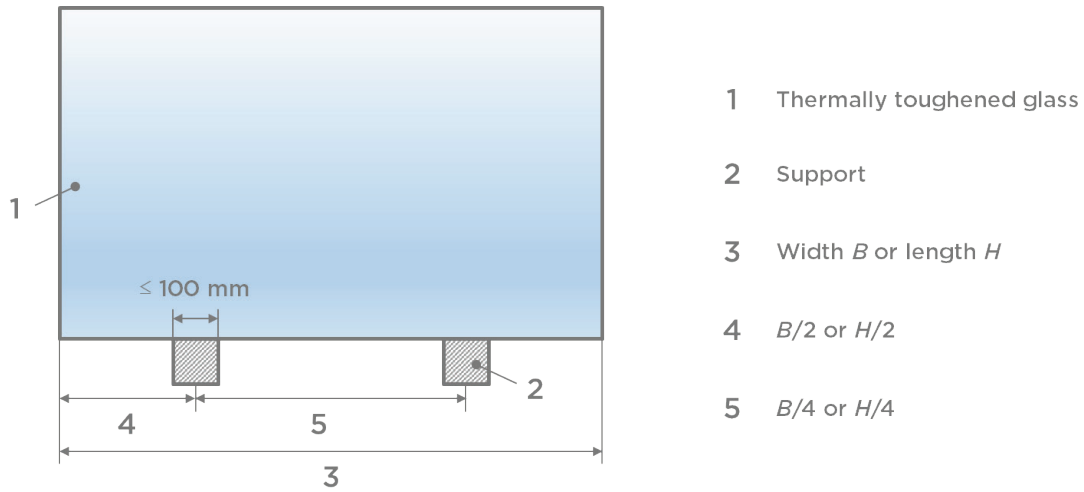
Picture 20: Support conditions for the measurement of overall bow
