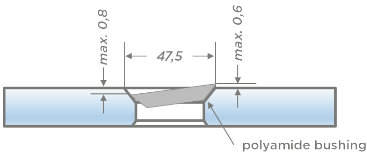
Picture 29: Schematic representation of possible mounting positions of e.g. MULTI-POINT fittings, 90° countersunk [Dimensions in mm]
