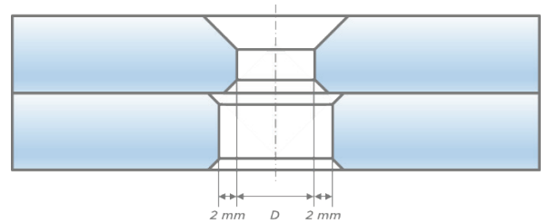
Picture 24: Countersunk holes in laminated glass
