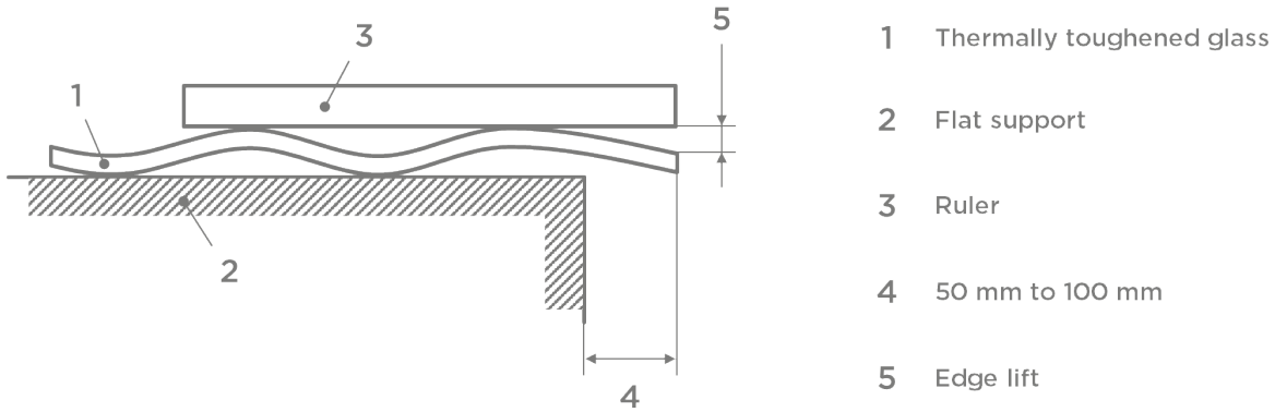
Picture 22: Measurement of the edge lift
