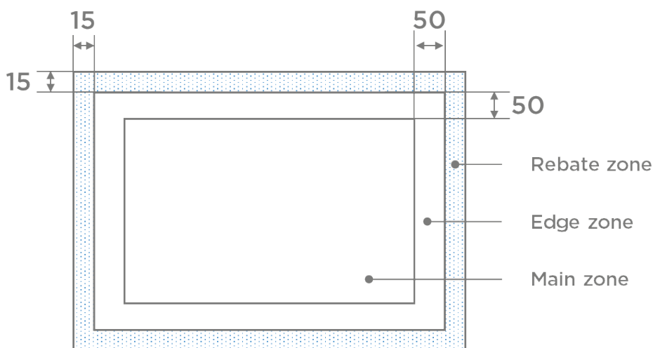
Picture 6: Zones for the assessment of visual quality [dimensions in mm]
