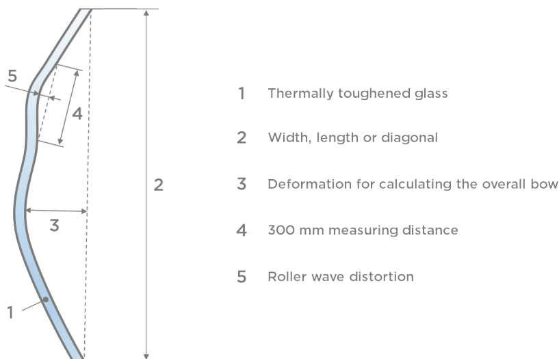
Picture 19: Representation of the overall bow and the roller wave distortion
