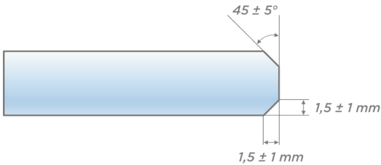
Picture 9: Chamfer tolerance for edge machining [ECKELT Standard]
