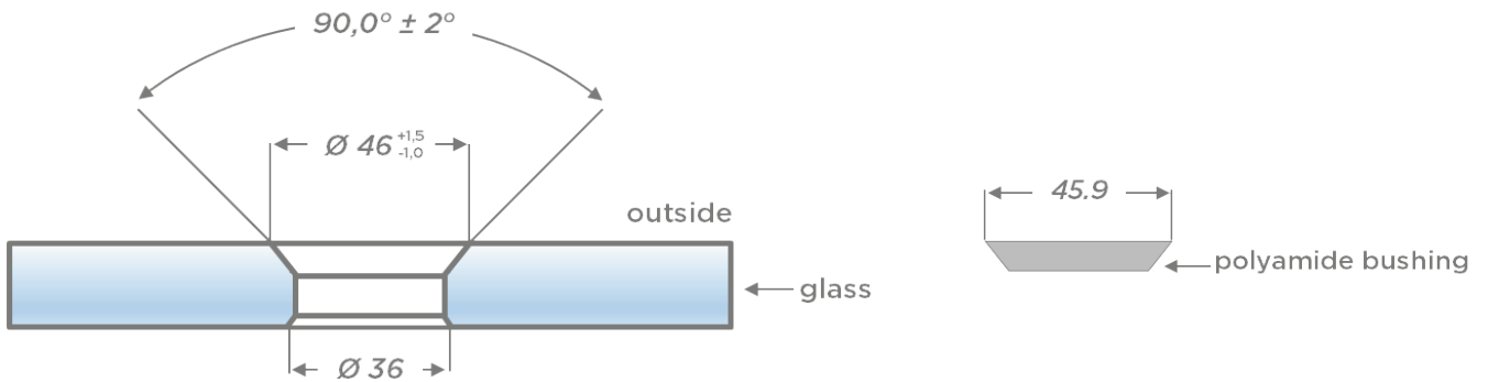
Countersunk hole nominal dimensions and tolerances
