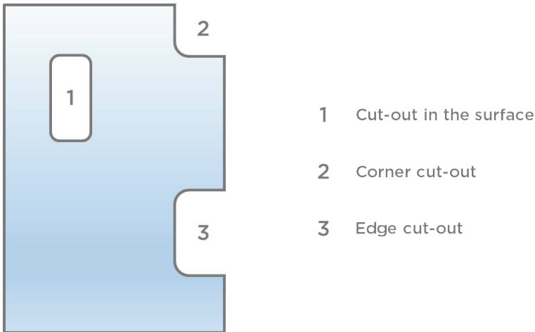
Picture 12: Different types of cut-outs
